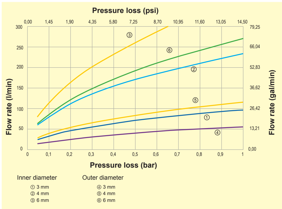
Figure 1: Max. flow rate for pneumatic contacts with shut-off
