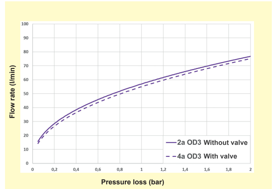
Figure 2: Comparing a female module with/without the shut-off valve
