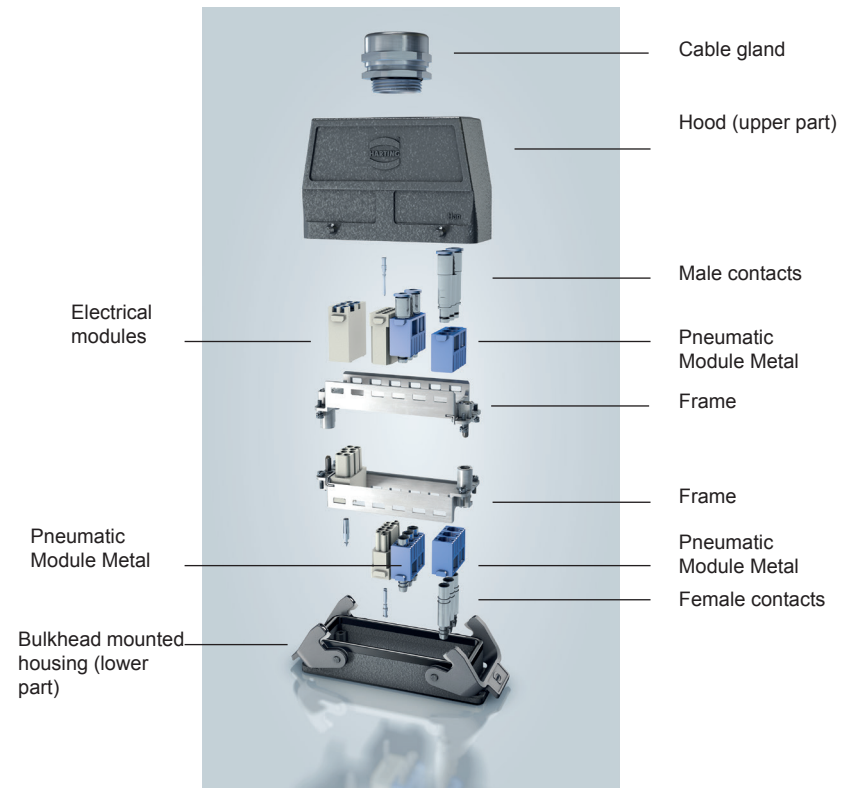
Figure 1: Assembly method for the Han-Modular® system
