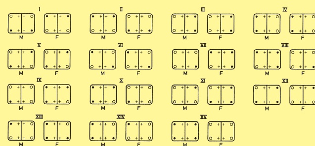
Figure 3: Connector with two frames
